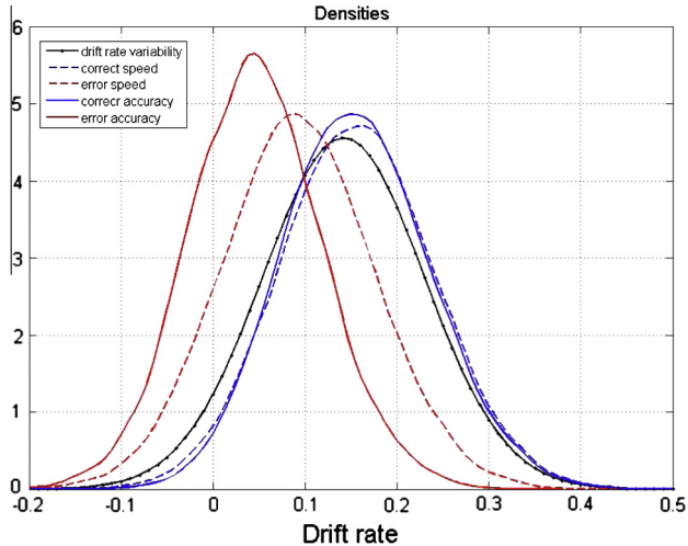
Fig. B1. Drift rate variability density curves across all trials (black) and conditional on correct (blue) and error (red) responses. Solid and dashed curves correspond to stress on choice accuracy and speed respectively. It can be clearly observed that the sum of the means for the correct and error curves, which constitutes the second stage resolution rate, is larger for the accuracy stress. Indeed, for correct responses the means are very similar whereas for error response the 'speed' mean is larger than the 'accuracy' mean. (For interpretation of the references to color in this figure legend, the reader is referred to the web version of this article.)
